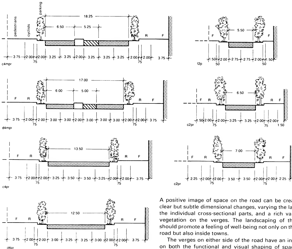
② Standard cross-sections for roads in built-up areas
